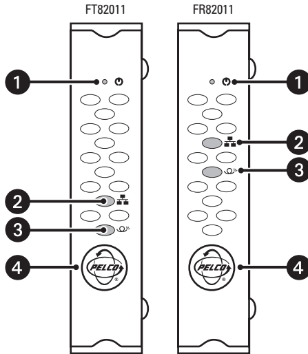
Figure 2. Front Panel of FT82011 and FR82011 Modules
